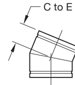
FIGURE 312 FABRICATED 22-1/2° ELBOW (SEGMENT WELDED)
