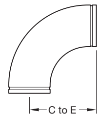
FIGURE 310LR FABRICATED 90° LONG RADIUS ELBOW
