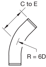
FIGURE 301-6D (45°)
