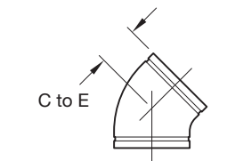
FIGURE 301 FABRICATED 45° ELBOW
