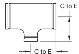
FIGURE 221 CAST REDUCING TEE
