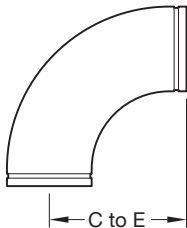
FIGURE 310 FABRICATED 90° ELBOW
