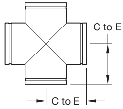
FIGURE 327 FABRICATED CROSS
