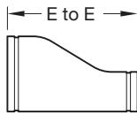
FIGURE 351 FABRICATED ECCENTRIC REDUCER (SEGMENT WELDED)
