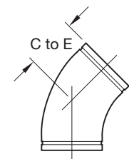
FIGURE 301LR FABRICATED 45° LONG RADIUS ELBOW
