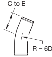
FIGURE 312-6D (22.5°)
