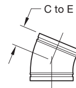
FIGURE 212 CAST 22-1/2° ELBOW
