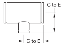
FIGURE 321 FABRICATED REDUCING TEE (SEGMENT WELDED)
