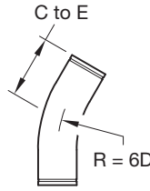
FIGURE 303-6D (30°)
